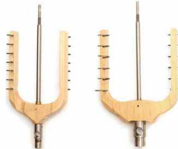
STANDARD FLYER ORIFICE 10 MM (3/8 IN)
